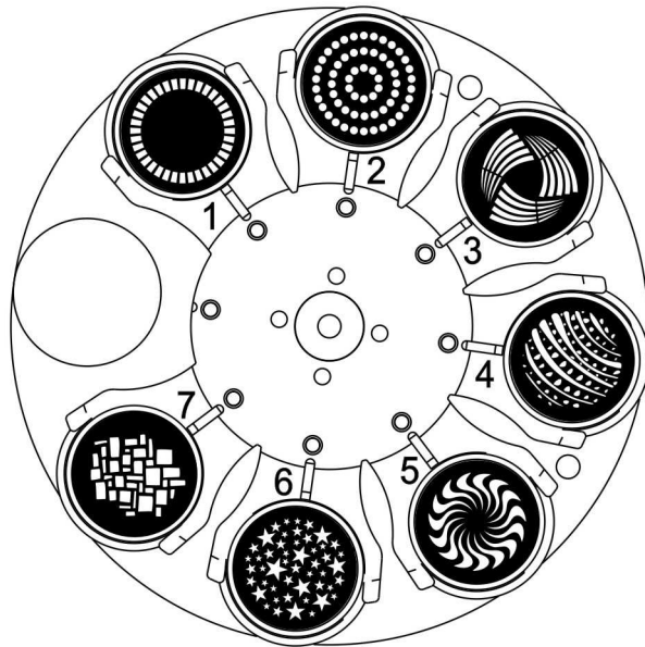
Fixation gobos wheel
